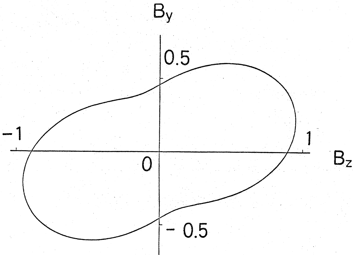
Fig. 2. The trajectory for a wave with periodicity in the (B_y, B_z) plane. A^2 = \alpha^2 = 0.2 , \epsilon = 0.5 , c = 0 , P_0 = 0.374 \dots , \underline{b_{00}} = 0.5 .
