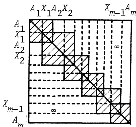
Fig. 5. A distance matrix corresponding to a cascade network.
