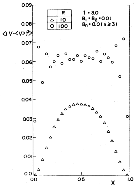
Fig. 20. Velocity variance field of the stochastic secondary flow with "red" noise.
