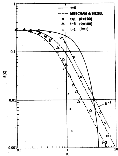
FIG. 6. Energy spectrums E(k, t) for various values of R and t with N = 30 .
