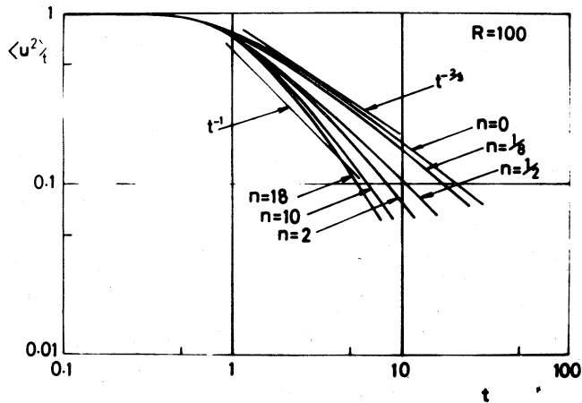
Fig. 7 Energy decay of Burgers equations with various initial energy spectrums.
