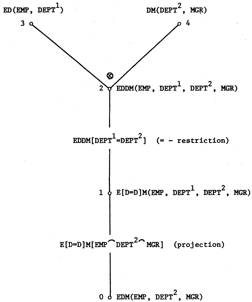
Fig. 1. The view defining tree of the view EDM.
