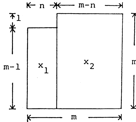
Fig.2. (m,n) -chunk.
