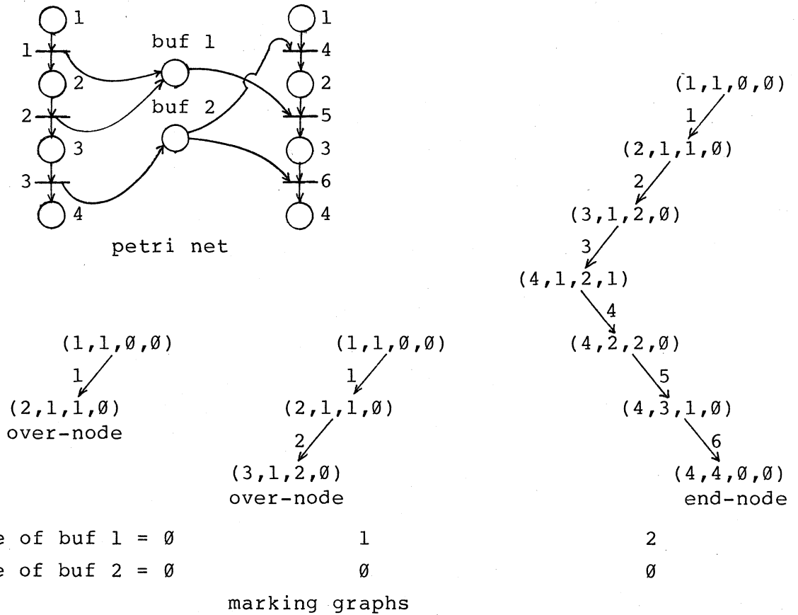
Figure 10. Analysis of buffer size.
