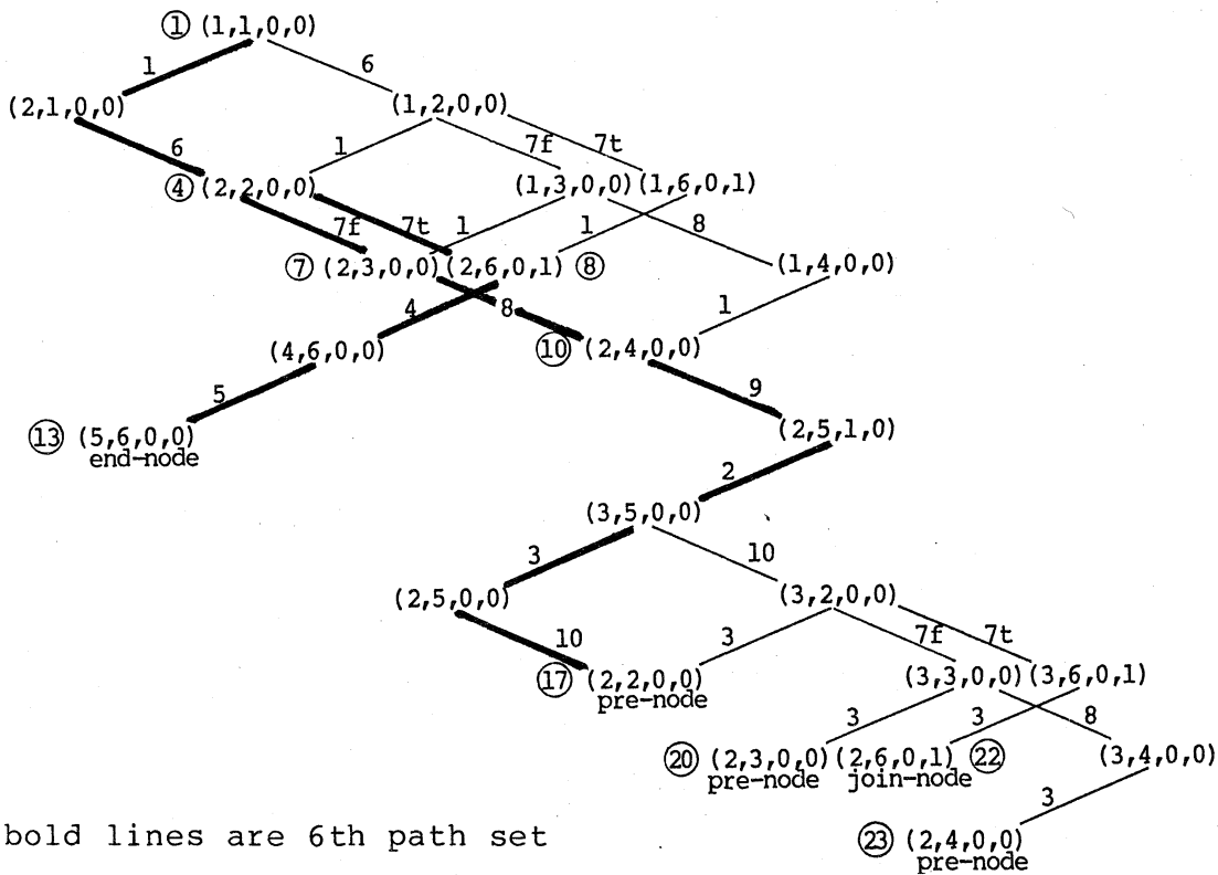
Figure 11. Marking graph for the Petri net of Figure 5. (buffer size = \emptyset )
