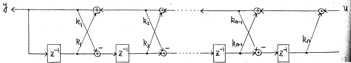
Fig. 2 Unnormalized Lattice Filter
