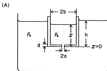
Figure 8 (A) Hydrodynamic oscillator with a plastic cup. (B) Experimental apparatus to monitor the interference between the two hydrodynamic oscillators.
