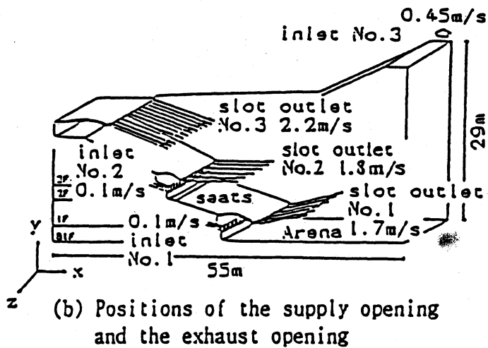
Fig.2 Plan of gymnasium and arrangement of supply and exhaust openings
