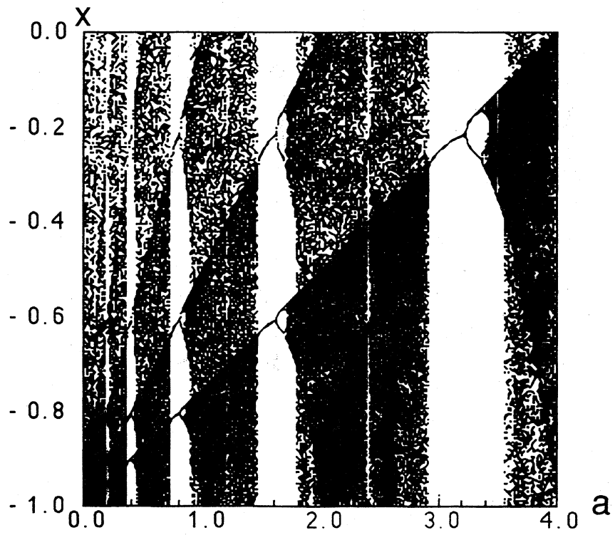
Fig. 11. Bifurcation diagram for Eq. (12), where \alpha = 0 .
