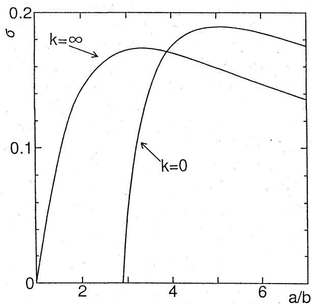
Fig. 5 Growth rate of the elliptical instability and the two-dimensional ( m=2 ) instability of the Moore-Saffman elliptic vortex. The horizontal axis is a/b . The vertical axis denotes the growth rate \sigma .
