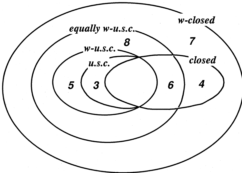
Figure 1: Relationship among Various Upper Semicontinuity Properties of Set-Valued Maps.
