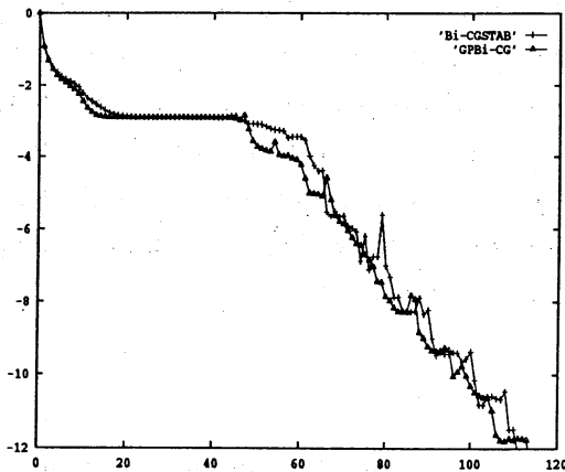
FIG. 2. The history of the residual 2-norms (i. e., \log(\|r_n\| / \|r_0\|) ) vs. n ) for example 1 ( \gamma = 2 )
