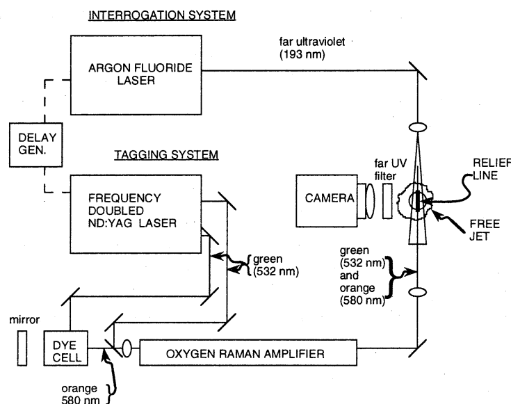
Figure 1. Block diagram showing the RELIEFsystem.
