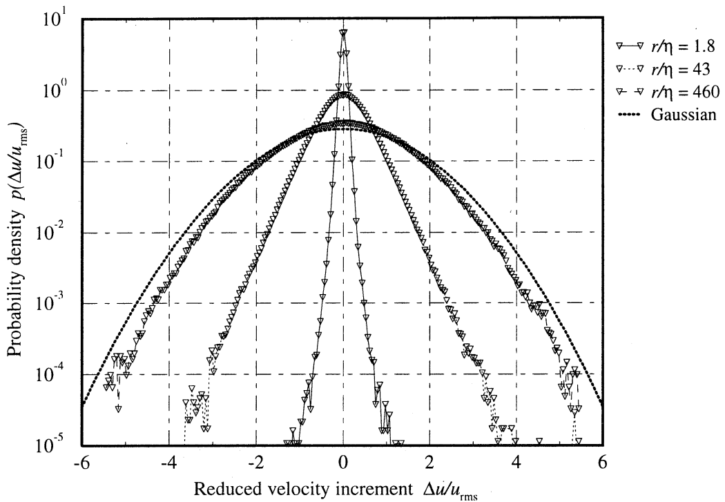
Figure 14. pdf of transverse velocity increments reduced by u_{\text{rms}} . Otherwise, as in Fig. 13.
