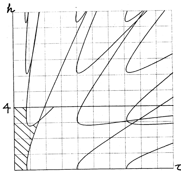
Fig. 3.2 (Case 1; a = -2 , b = \frac{1}{2} )
