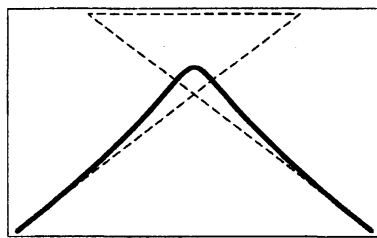
(a) A parametric cubic curve
