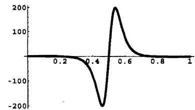
(c) Derivative of curvature plot
