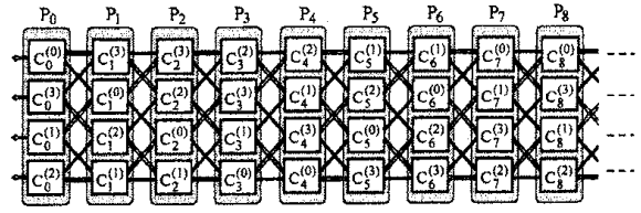
Figure. Systolic array for codes on C_4^{11} curves
