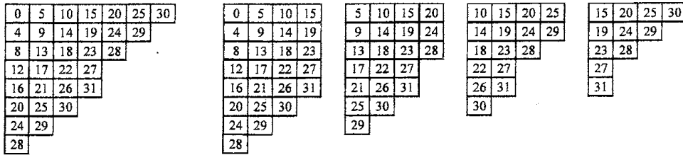
Figure. Pole orders on \Phi(7, 31) and \Phi^{(i)}(4, 31) ( 0 \leq i \leq 3 )
