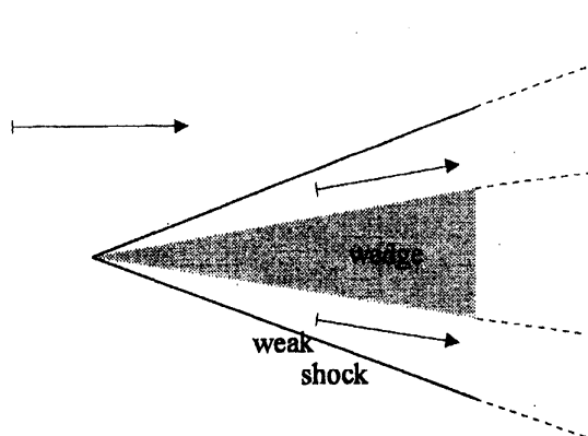
Figure 1: Weak shock
