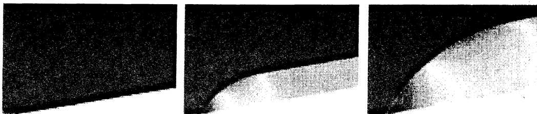
Figure 6: The weak shock appears spontaneously at the corner. It is connected to the straight reflected shock by a curved shock, with a nontrivial elliptic region below.
