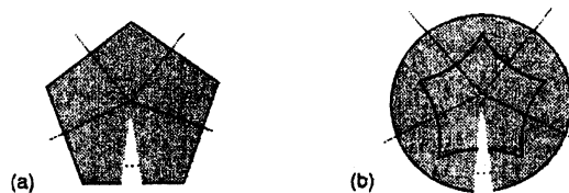
Figure 9: (a) image of the moment map, and (b) the planar portrait of a regular toric surface
