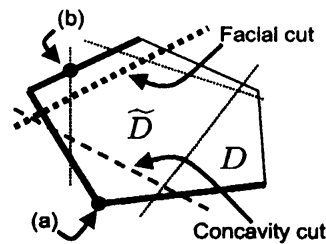
Figure 3: A 0-dimensional face (a) and three proper faces (bold solid lines) of D are identified in \tilde{D} . If the corner (a) is found in Step 2, a concavity cut is constructed. If the corner (b) is found, a facial cut is constructed. If these two cuts are added to \tilde{D} , the remaining area includes no face of D .
