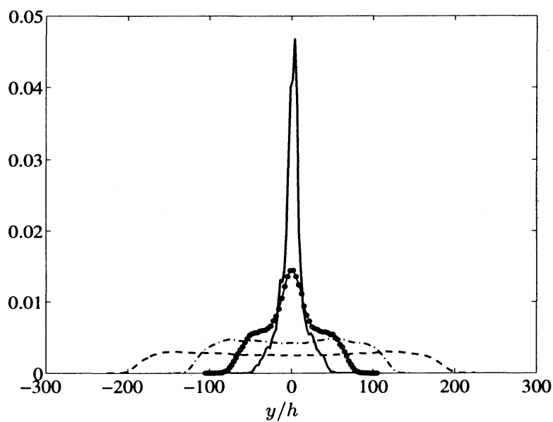
Figure 13: The PDF of the position of low-velocity streaks on the duct wall: —, Re_b = 1100 ; —○—, Re_b = 1500 ; ···, Re_b = 2200 ; ----, Re_b = 3500 .
