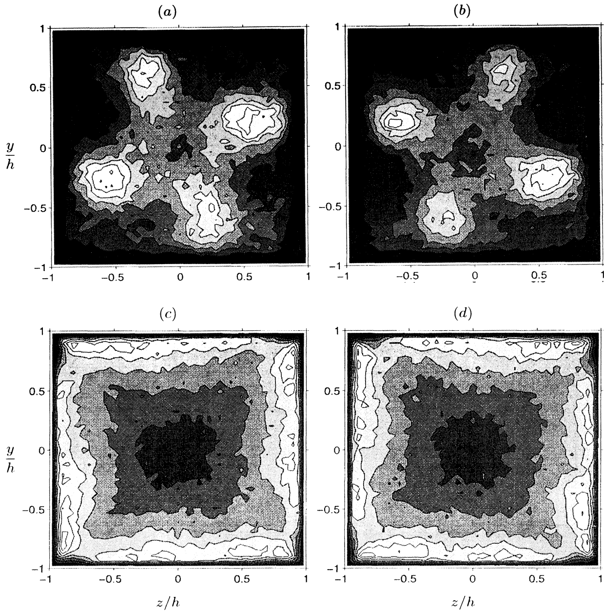
⊠ 11: The PDF of the position of vortex centers: (a), (b) Re_b = 1100 ; (c), (d) Re_b = 2200 ( L_x/h = 4\pi ). (a), (c) vortices with positive (clockwise) streamwise vorticity; (b), (d) negative (counter-clockwise) streamwise vorticity.
