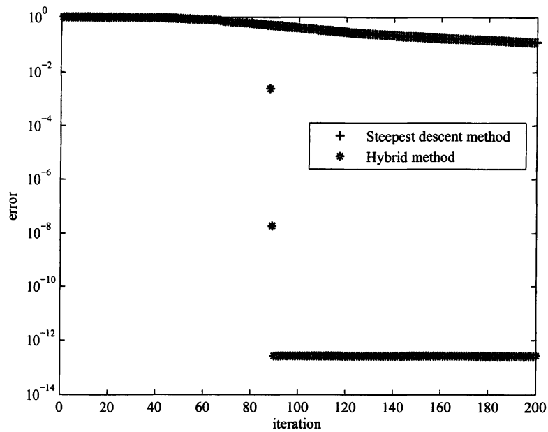
図 5.1: n = 300, p = 150 .
