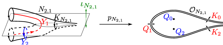
FIGURE 1. The involution \iota_{N_{2,1}} of N_{2,1}
