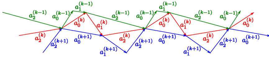
FIGURE 4. Adjacent complex probabilities of \rho_1 \in \Omega(\Sigma_{1,1})
