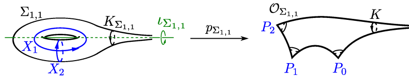
FIGURE 2. The involution \iota_{\Sigma_{1,1}} of \Sigma_{1,1}
