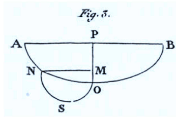
fig.1 a meniscus in a canal.
