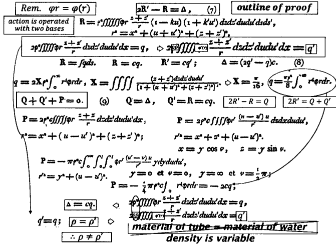
fig.2 Outline of proof by Poisson on the abrupt variation causing the rise in the neighborhood of water surface and wall.
