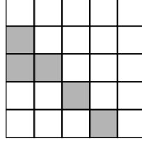
FIGURE 2. h = (3, 3, 4, 5, 5) のとき, \dim_{\mathbb{C}} \text{Hess}(N, h) = 5
