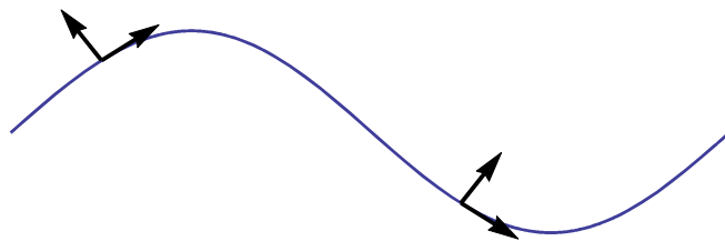
Figure 1: An inextensible planar string.
