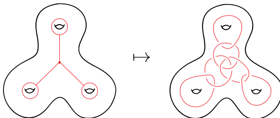
Figure 3: Framed link associated to a degree 1 clasper.
