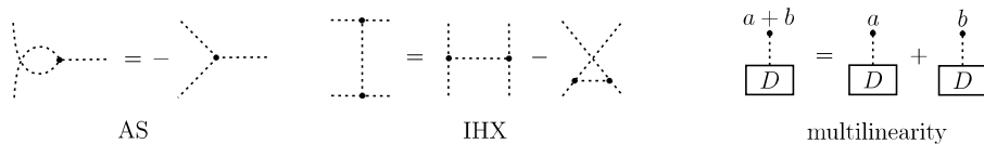
Figure 6: Relations in \mathcal{T}(C) . Here a, b \in C .
