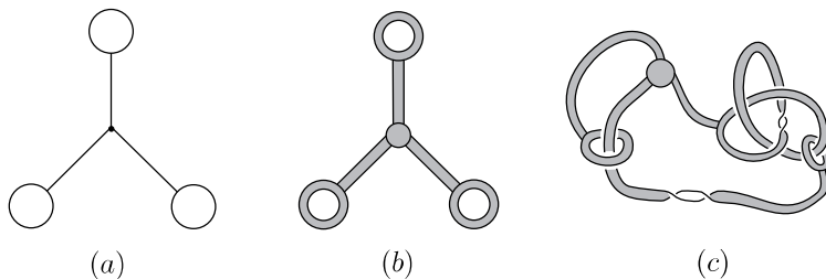
Figure 2: (a) Graph G . (b) Thickening \mathbb{G} . (c) Embedding \mathbb{G} \hookrightarrow M .
