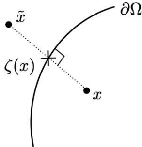
Figure 4: Picture of \zeta(x) and \tilde{x} .
