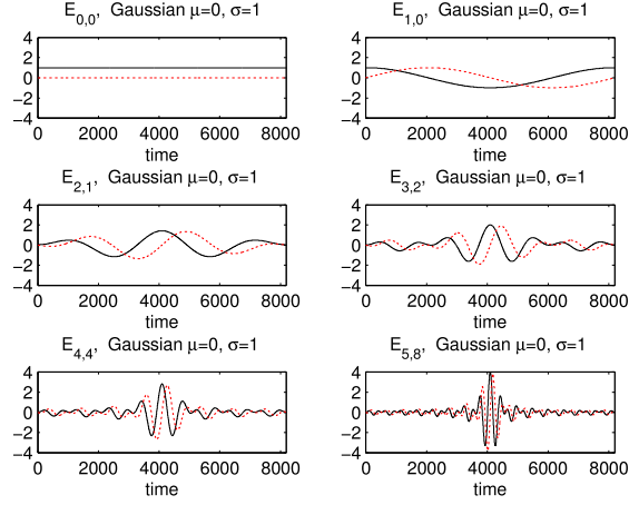
FIGURE 3. E_{p,\tau}^\varphi basis functions in increasing frequency p -bands. Black line = real, red line = imaginary. \hat{\varphi} is a Gaussian window with \mu = 0 and \sigma = 1 . Notice the similarities with Figure 1.
