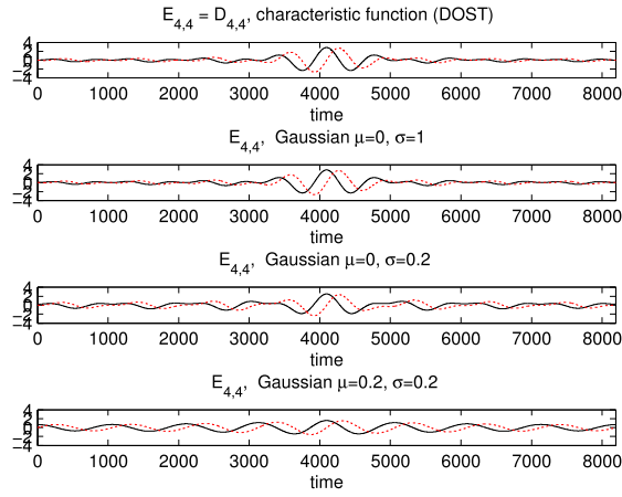
FIGURE 5. E_{p,\tau}^\varphi basis functions with p = 4 and \tau = 4 with different windows. Black line = real, red line = imaginary. \hat{\varphi} are \chi_{[-1/3,1/3]} or truncated Gaussian windows with varying \mu and \sigma .
