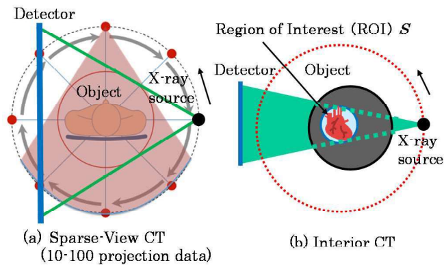
Fig. 1 Principles of sparse-view CT and interior CT.
