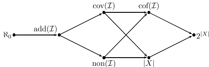
Figure 1: Diagram of the cardinal characteristics associated with \mathcal{I} . An arrow \aleph \rightarrow \eta means that (provably in ZFC) \aleph \leq \eta .
