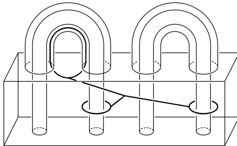
Figure 1: Clasper in \Sigma_{2,1} \times [-1, 1] .
