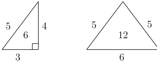
Figure 1: Heronian Triangles
