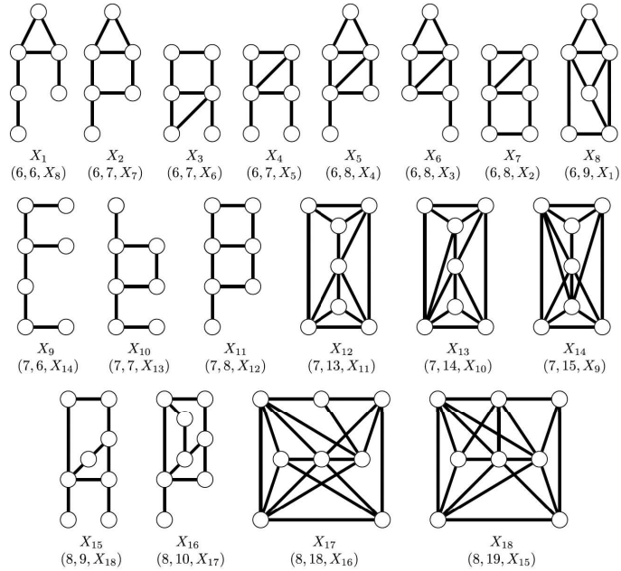
Figure 3: Minimal asymmetric graphs
