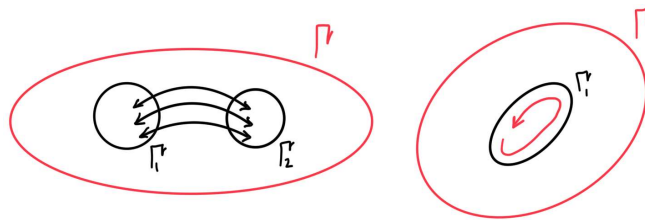
Figure 2: Two situations for partial automorphism of a graph.
