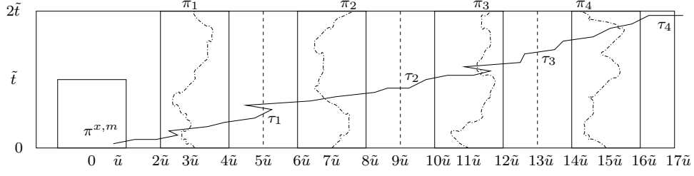
Figure 1: The random walks \pi_1, \pi_2, \pi_3 and \pi_4 start from 3\tilde{u}, 7\tilde{u}, 11\tilde{u} and 15\tilde{u} at time 0 and each stays within a distance of \tilde{u} . The random walk \pi^{x,m} starts from (x, m) inside the rectangle R(0, 0; \tilde{u}, \tilde{t}) and exits the right boundary of the rectangle R(0, 0; 17\tilde{u}, 2\tilde{t}) at time \tau_4 without coalescing with \pi_1, \pi_2, \pi_3 and \pi_4 on the way.
