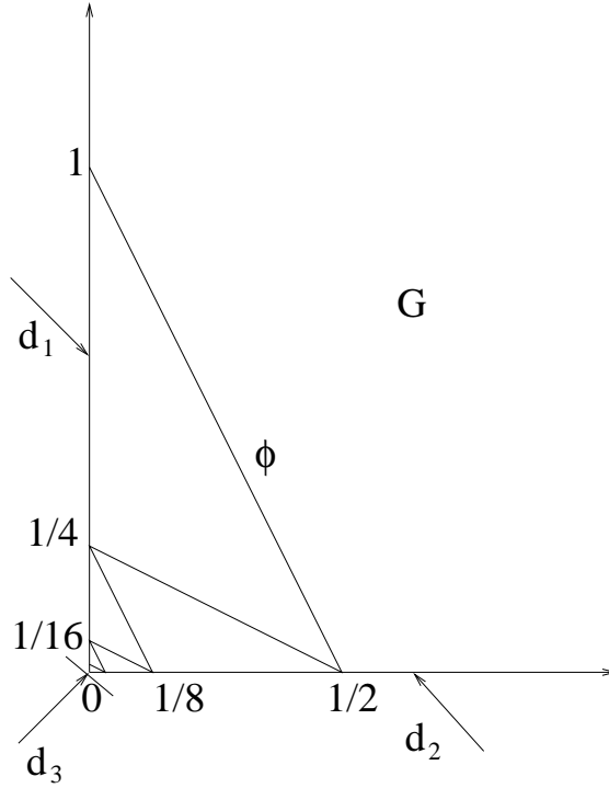
Figure 2: The solution (\phi, \eta) to the 2-dimensional GPS ESP with |\eta|(\tau_0) = \infty
