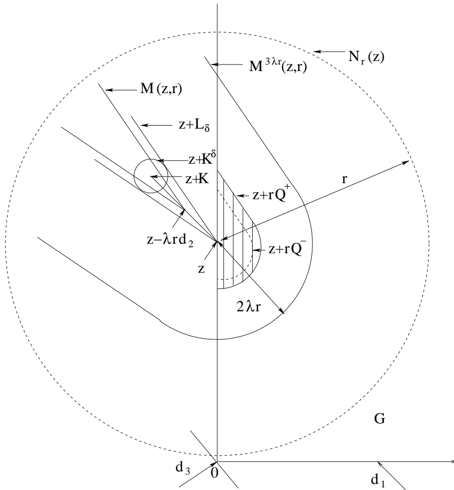
Figure 3: Construction of g_{z,r} for the 2-dimensional GPS ESP
