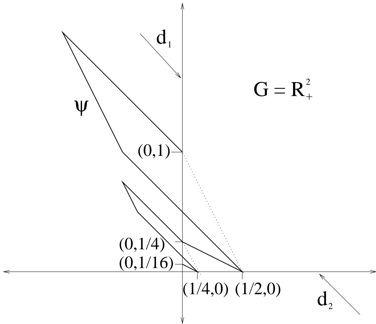
Figure 1: An input trajectory \psi for the 2-dimensional GPS ESP
