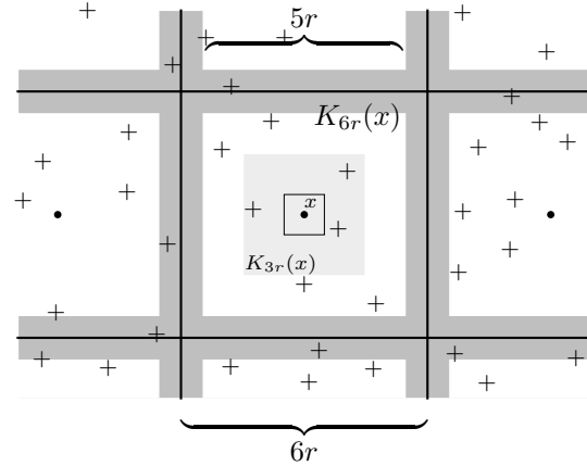
Figure 1: Matérn hard-core process type I: Given that the process \Phi is known on the borders \cup_{l \in \mathcal{M}} K_{6r}(x_l) \setminus K_{5r}(x_l) (grey area), the boxes \Phi|_{K_{6r}(x_l)} , l \in \mathcal{M} , are independent.
