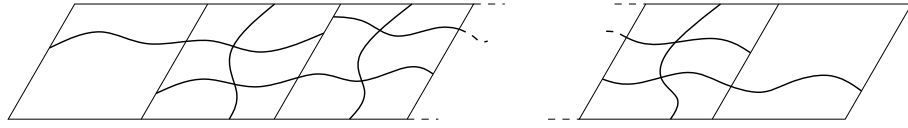
Figure 3: This construction shows that we can take f_k(\delta) = \delta^{k-2}(f_2(\delta))^{k-1} .
