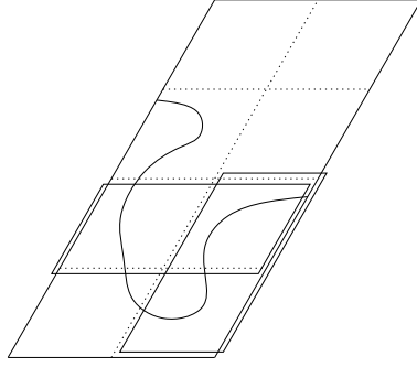
Figure 16: Two of the small sub-parallelograms are crossed in the “easy” way.
