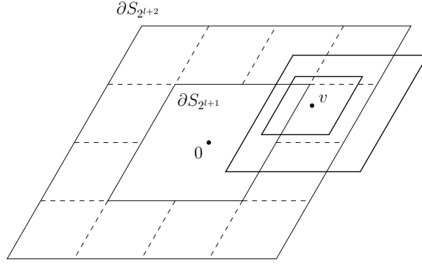
Figure 13: We replace R(v) = S_{2^l}(v) by one of the \tilde{R}_{2^{l+1}}^i ( i = 1, \dots, 12 ).
