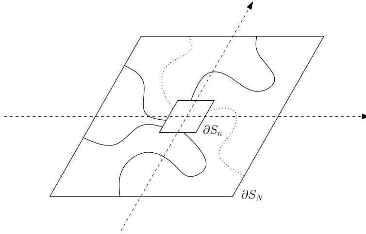
Figure 5: The event A_{6,\sigma}(n, N) , with \sigma = BBBWBW .
