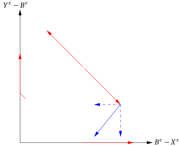
Figure 3: The particle's jumps (red arrows) are parallel to the level lines of the \|\cdot\|_1 -norm. In the sense of this norm, it can increase on the axes only. The drift consists of two independent components (blue dashed arrows), which are orthogonal to the axes. The resulting drift is illustrated by the solid blue arrow.
