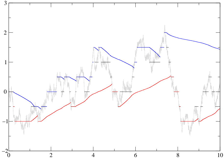
Figure 2: The three processes B^\epsilon (black), X^\epsilon (red) and Y^\epsilon (blue); B is displayed beneath in grey. \epsilon = 1/2 in this figure.
