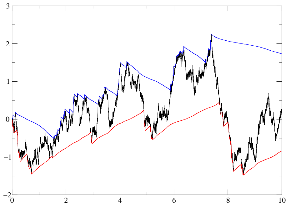
Figure 1: The price B (black), and the opinions X (red) and Y (blue) evolving in time on a logarithmic scale.
