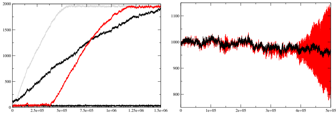
Figure 6: The left graph shows the gap of the system for different \gamma . Being stable for \gamma = 1.5 (black lower graph), it increases for \gamma = 1.6 (red) and \gamma = 1.7 (grey). However, if the system is started with \gamma = 1.5 but with an artificially enlarged gap, it also increases (black increasing graph). The convergence to a value below 2000 is due to a restriction of the state space in the numerical simulations. The right graph shows the stable, respectively unstable, behaviour for \gamma = 1.5 (black) and \gamma = 1.6 (red) in terms of the price process.
