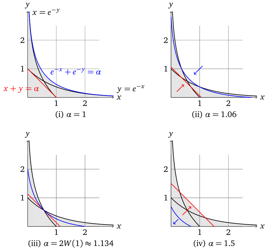
Figure 6: The dynamics of the shaded region R(\alpha) : (i) At \alpha = 1 , the boundary of R(\alpha) is given by the blue curve e^{-x} + e^{-y} = 1 and the area is \pi^2/6 . (ii) The area of R(\alpha) decreases with \alpha as the curve e^{-x} + e^{-y} = \alpha moves towards the origin. (iii) At \alpha = 2W(1) , the four curves meet in the point (W(1), W(1)) and the area of R(\alpha) reaches its minimum. (iv) For larger \alpha , the area of R(\alpha) increases as the red curve x + y = \alpha moves up and to the right.
