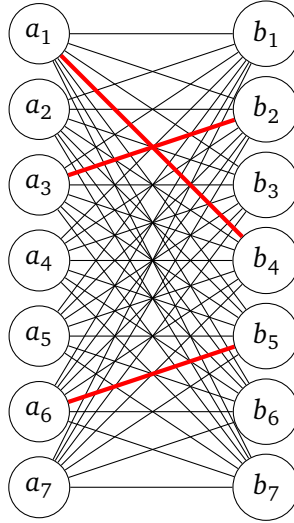
Figure 4: The complete bipartite graph whose vertex sets are the elements of the two Fano matroids. The red edges constitute one of the solutions to the 3-flow problem.
