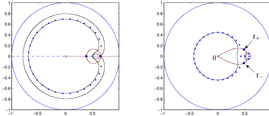
FIG. 2.3. Left: zeros of \Phi_n for w given in (2.30) with \rho = 1/2 and n = 30 , along with the level curves \text{Re}(\Psi_n(z) - \Psi_n(t_+)) = 0 , \text{Re}(\Psi_n(z) - \Psi_n(t_+)) = \frac{1}{n} \log\left(\frac{1}{2\sqrt{\pi}} \frac{\rho^{3/4}}{n^{3/4}}\right) and \text{Im}(\Psi_n(z) - \Psi_n(t_+)) = 0 . Right: the same, but for the weight 1/w . Observe that the level curve (2.32) has now two components.
