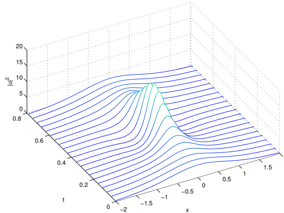
FIG. 4.1. Breather solution for the focusing NLS equation.
