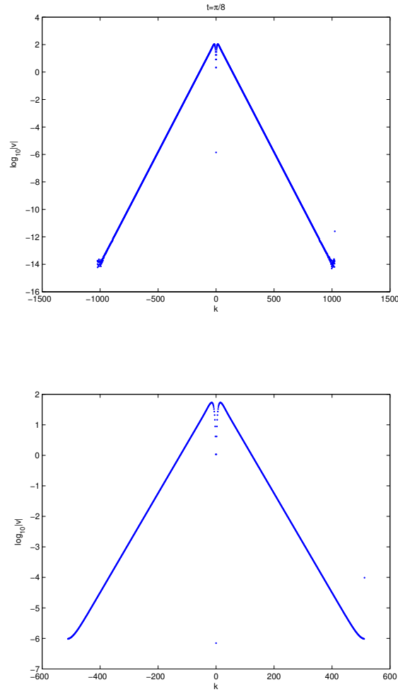
FIG. 6.3. Breather solution to the focusing NLS equation at t = \pi/8 . The plots show the Fourier coefficients v in dependence of the spatial frequencies k for 2^{11} (top) and 2^{10} (bottom) points.
