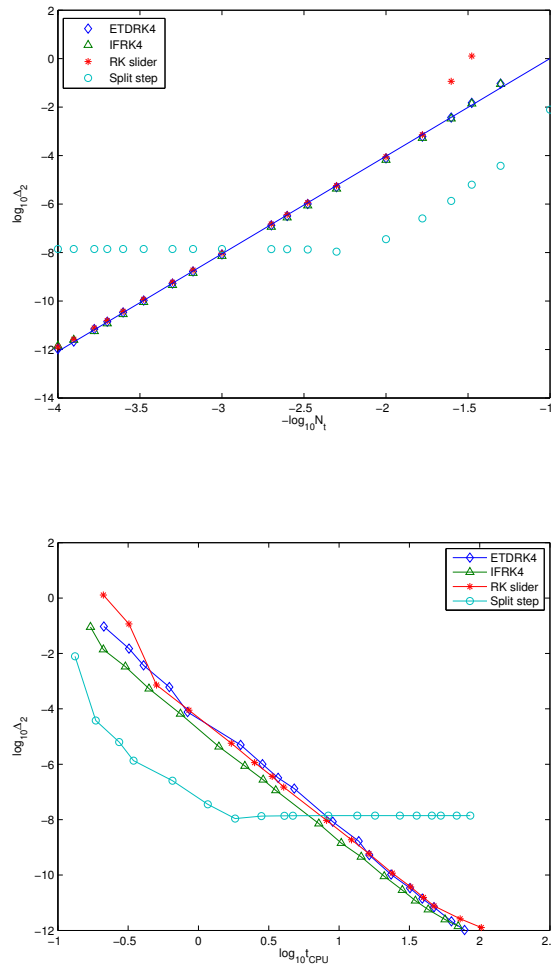
FIG. 4.6. Normalized L_2 norm of the numerical error for several numerical methods, as a function of N_t (top) and as a function of CPU time (bottom). The shown straight line has slope 4.0.
