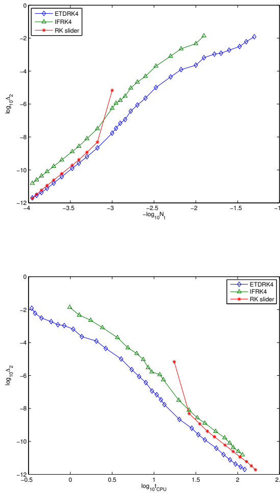
FIG. 3.4. Normalized L_2 norm of the numerical error for several numerical methods, as a function of N_t (top) and as a function of CPU time (bottom).
