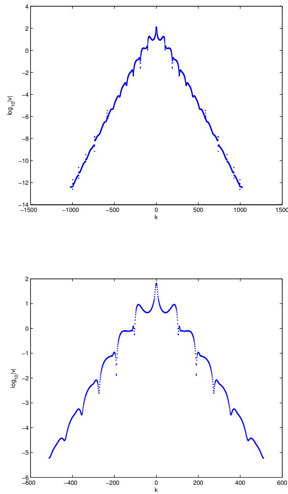
FIG. 6.1. Solution to the KdV equation with \epsilon = 0.1 for the initial data u_0 = -\text{sech}^2 x at t = 0.4 . The plots show the Fourier coefficients v in dependence of the spatial frequencies k for 2^{11} (top) and 2^{10} (bottom) points.
