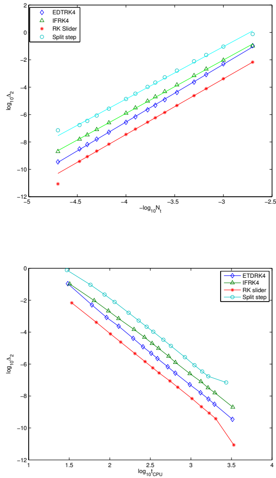
FIG. 4.4. Normalized L_2 norm of the numerical error for several numerical methods, as a function of N_t (top) and as a function of CPU time (bottom). The shown straight lines have slope 4.1 for RK sliders, 3.8 for split step, 3.9, for the integrating factor method, and 4.2 for ETD.
