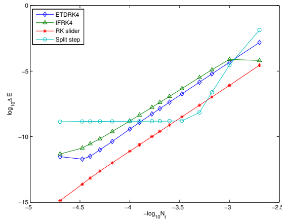
FIG. 5.2. Normalized violation of energy conservation for the focusing NLS solution with initial data u_0 = \exp(-x^2) and \epsilon = 0.1 for several numerical methods. The shown straight line has slope 5.1.
