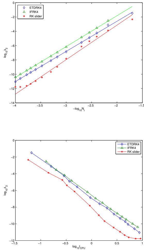
FIG. 3.1. Normalized L_2 norm of the numerical error for several numerical methods, as a function of N_t (top) and as a function of CPU time (bottom). The shown straight lines have slopes 4.8 for RK sliders, 4.3 for the integrating factor method and for ETD.
