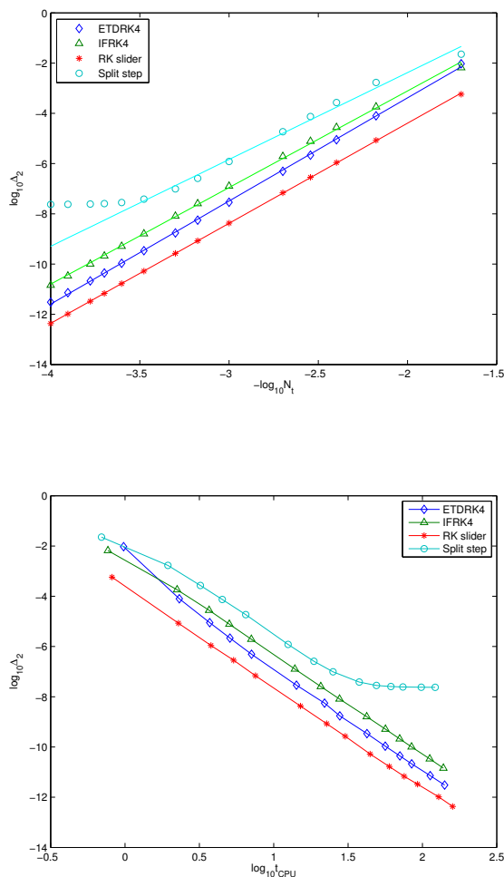
FIG. 4.2. Normalized L_2 norm of the numerical error for several numerical methods, as a function of N_t (top) and as a function of CPU time (bottom). The shown straight lines have slope 4.0 for RK sliders, 3.5 for split step, 3.9 for the integrating factor method, and 4.1 for ETD.
