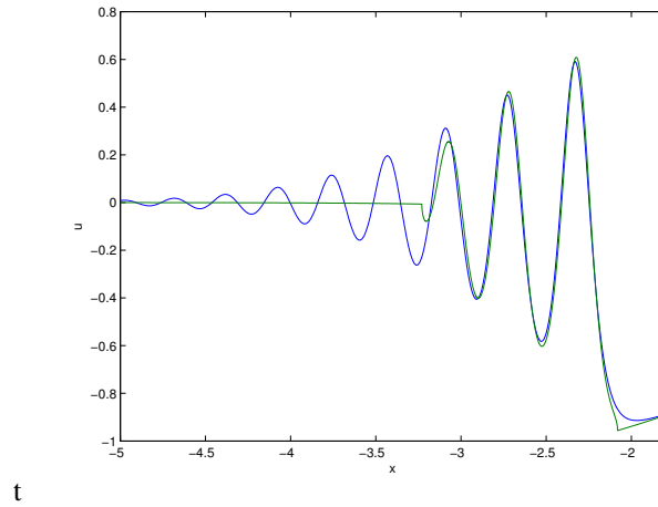
FIG. 1.1. The blue graph shows the solution to the KdV equation for \epsilon = 0.1 for the initial data u_0(x) = -\text{sech}^2 x at the time t = 0.4 , the green graph the corresponding asymptotic solution according to [28, 39, 13].
