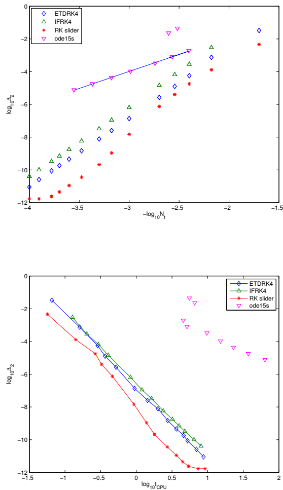
FIG. 3.2. Normalized L_2 norm of the numerical error for several numerical methods, as a function of N_t (top) and as a function of CPU time (bottom). The shown line has slope 2.08.
