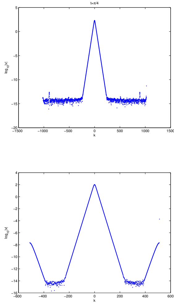
FIG. 6.2. Breather solution to the focusing NLS equation at t = \pi/4 . The plots show the Fourier coefficients v in dependence of the spatial frequencies k for 2^{11} (top) and 2^{10} (bottom) points.
