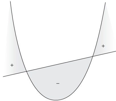
Figure 1: Graphic concept of Jensen's inequality.
