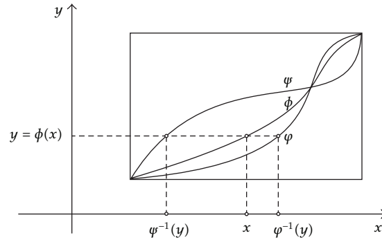
Figure 3: Convex combination of strictly monotone increasing functions \varphi and \psi .
