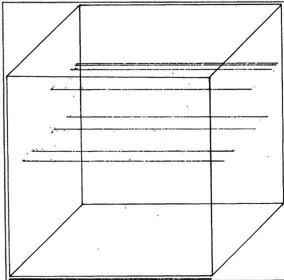
FIGURE 1 Rod-type dynamics of limited chaos; 10,000 iterations. See text for parameter specifications.
