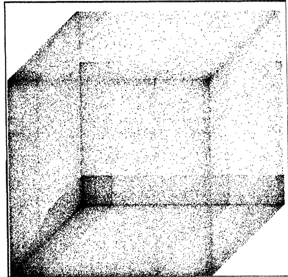
FIGURE 3 Chaotic dynamics in the unit cube in absence of attractors; 25,000 iterations. See text for parameter specifications.
