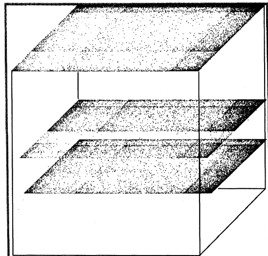
FIGURE 2 Sheet-type dynamics of limited chaos; 10,000 iterations. See text for parameter specifications.
