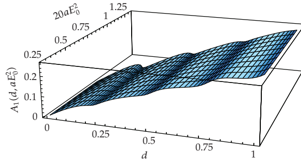
Figure 5: Absorptance A_1 depending on the layer thickness d and on the incident field intensity aE_0^2 for the same parameters as in Figure 3.
