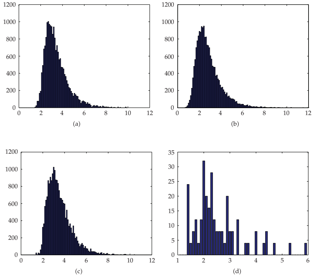
Figure 2: (a, b) the log-ratio histograms of all Costas permutations of order 15 (a) and an equinumerous collection of randomly chosen permutations of order 15 (b); Costas permutations are shown to be more nonlinear. (c, d) the log-ratio histograms of all Costas permutations of order 16 (c) and of all algebraically constructed Costas permutations of order 16 (d); algebraically constructed Costas permutations seem to be amongst the most linear ones.
