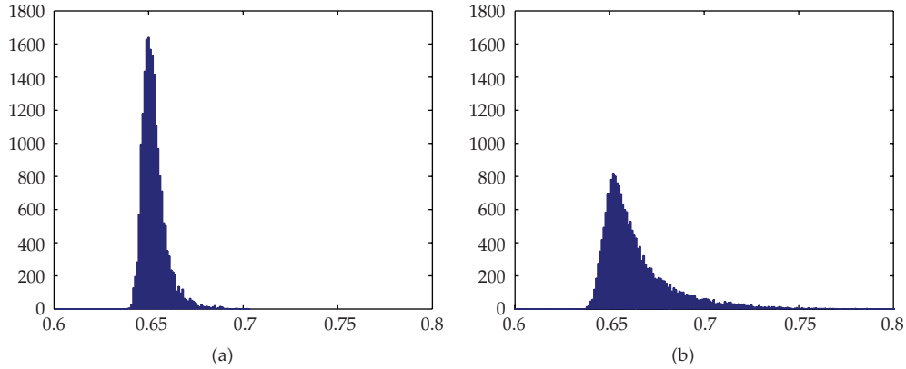
Figure 1: The histograms of all Costas permutations of order 15 (a) and an equinumerous collection of randomly chosen permutations of order 15 (b), according to \mathbb{L} : Costas permutations are shown to be more nonlinear.
