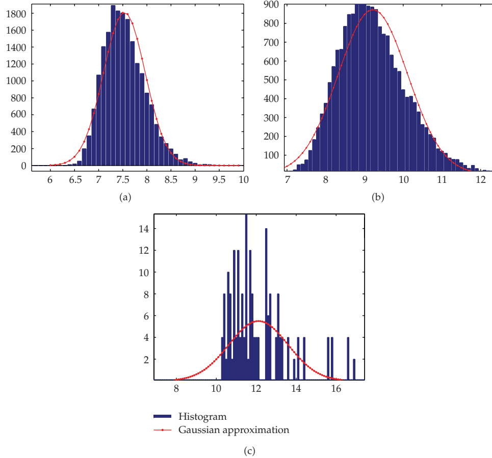
Figure 3: The linearity histogram of all Costas permutations of order 15 (a) is well approximated by the Gaussian of the same mean and variance, but the corresponding histogram of order 27 (c) is not, due to the small number of samples. Furthermore, the linearity criterion is efficient: histograms show that the linearity of Costas permutations of order 15 is clearly less than that of an equinumerous collection of randomly chosen permutations of order 15 (b).
