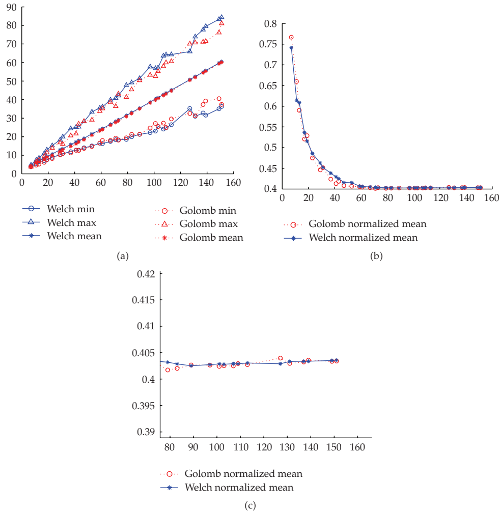
Figure 4: (a) plot of the minimal, maximal, and mean linearities for the Welch and Golomb family generated in \mathbb{F}(p) , 3 \leq p \leq 151 . (b) plot of the mean linearity divided by the order, indicating convergence near 0.4. (c) a detail of the tail of the previous plot.
