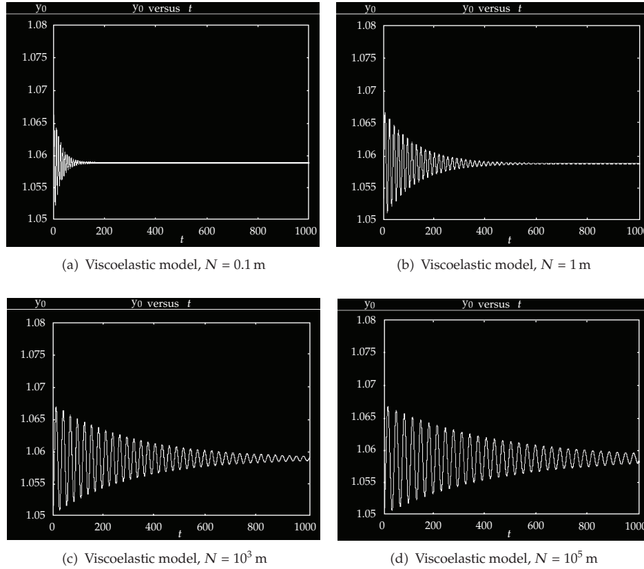
Figure 2: Stretch ratio with varying N .
