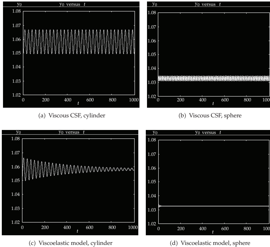
Figure 8: Stretch ratio for cylindrical versus spherical geometry.
