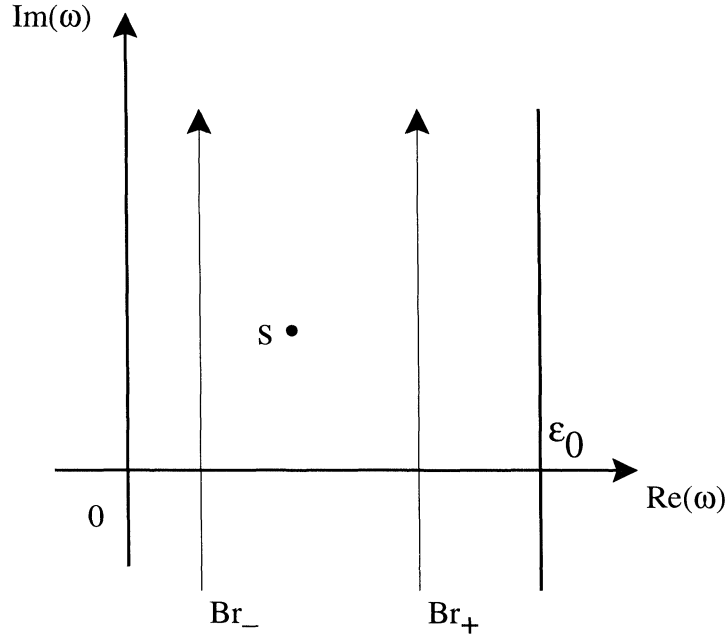
Figure 1. A sketch of the integration contours in the complex \omega -plane.
