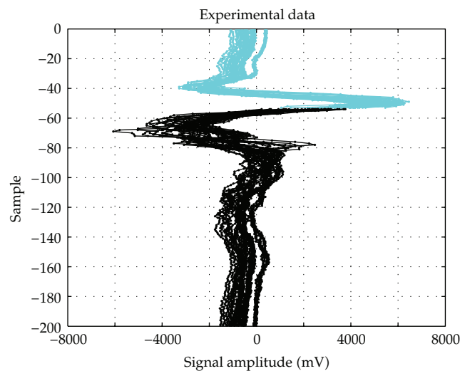
Figure 8: Experimental data of 2.3 GHz antenna: discarded samples in cyan and considered samples in black.
