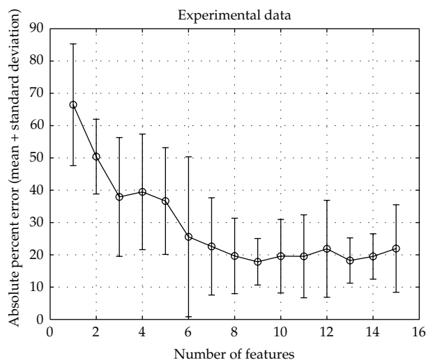
Figure 16: Absolute Error main results for PLP-MGM with PCA components of features extracted from experimental data of 2.3GHz antenna to approximate depth of inclusions.
