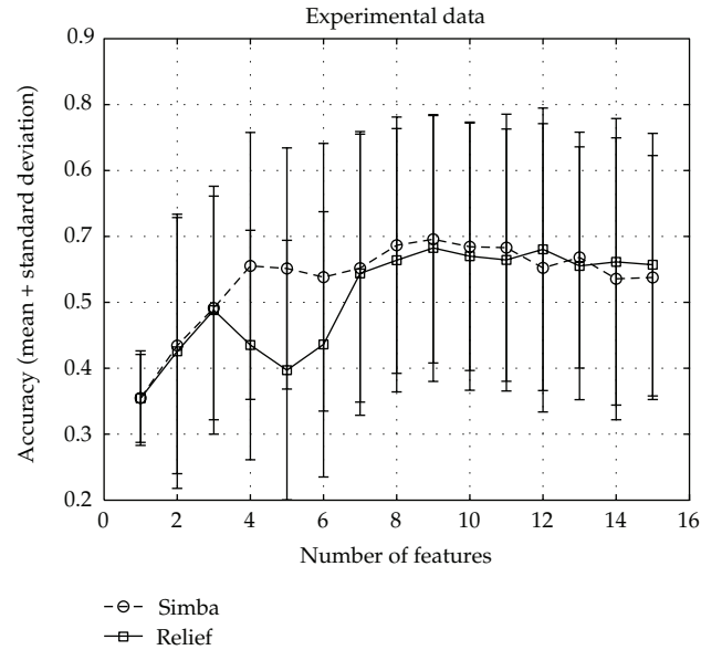
Figure 10: Accuracy results for k -NN with features extracted from experimental data of 2.3 GHz antenna to classify types of inclusions.
