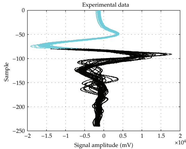
Figure 7: Experimental data of 1.6 GHz antenna: discarded samples in cyan and considered samples in black.
