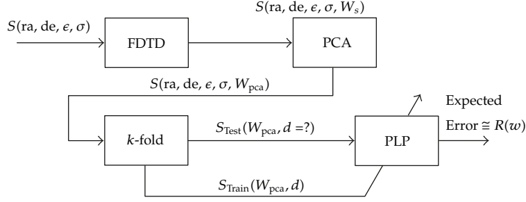
Figure 3: This figure shows an overview of the detection system employed using the ANN. Firstly, given a set S of radii ( ra ), depths ( de ), \epsilon_r , and \sigma a scattered wave ( W_s \in \mathbb{R}^p ) is calculated using FDTD. Afterwards, a dimensional reduction is applied. In the next step, the expected error is estimated to adapt the Parallel Layer Perceptron network parameters. In this work a 10-fold cross-validation was employed.
