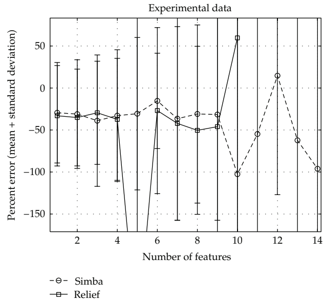
Figure 12: Percent Error main results for PLP with features extracted from experimental data of 2.3GHz antenna to approximate depth of inclusions.
