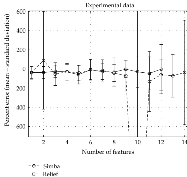
Figure 11: Percent Error main results for PLP with features extracted from experimental data of 1.6 GHz antenna to approximate depth of inclusions.
