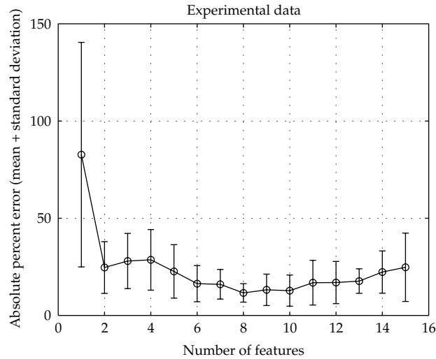
Figure 15: Absolute Percent Error main results for PLP-MGM with PCA components of features extracted from experimental data of 1.6 GHz antenna to approximate depth of inclusions.
