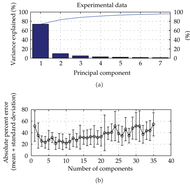
Figure 14: Absolute Error main results for PLP-MGM with PCA components of samples from experimental data of 2.3 GHz antenna to approximate depth of inclusions.
