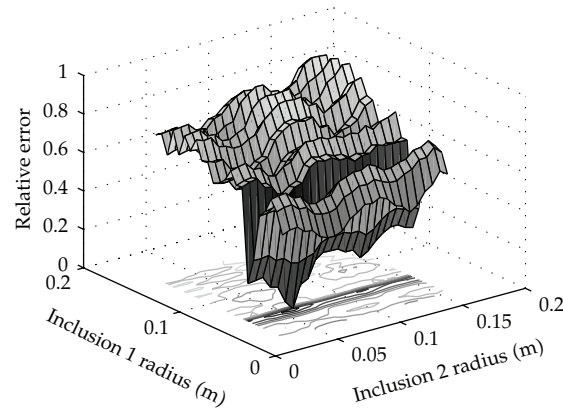
Figure 2: Surface plot of (3.1) representing the problem of finding the radii of two inclusions, given that their location and physical properties are known. Even in this simple example the surface is clearly multi-modal, thus, stochastic methods must be employed in the parametric approach.
