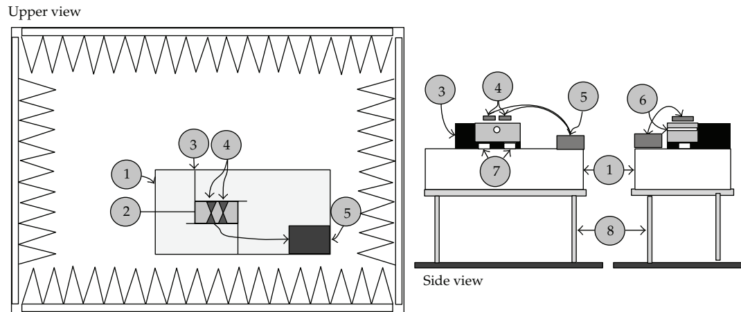
Figure 5: Schematic and photo of the assembly held in semi-anechoic chamber. (1) Polystyrene layer, (2) concrete block, (3) absorber plate, (4) bowtie antennas, (5) GPR control unit, (6) inclusion, (7) polystyrene blocks, and (8) wood table.
