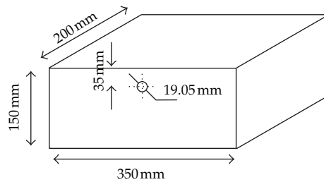
Figure 4: Concrete slab dimensions.
