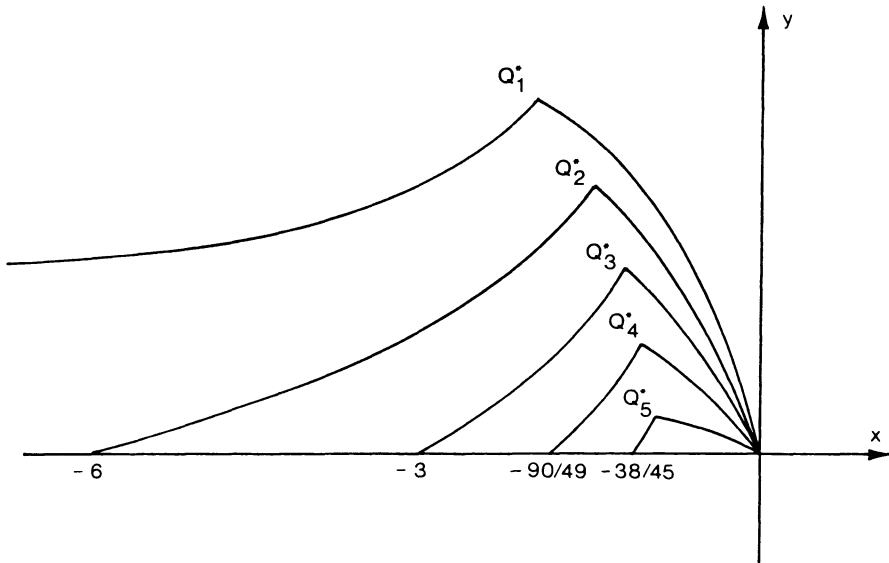
Fig. 2. Stability regions for Adams-Moulton methods for k=1,2,3,4,5 .
